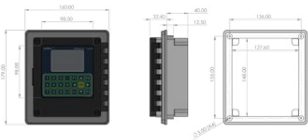
Ultra 4 Fascia-Mount Dimensions
