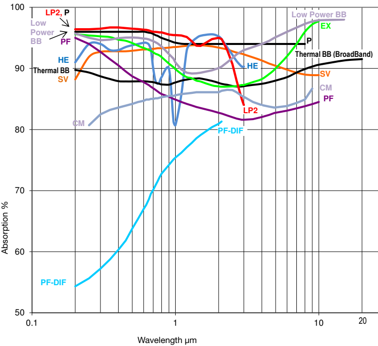
Absorption vs. Wavelength
