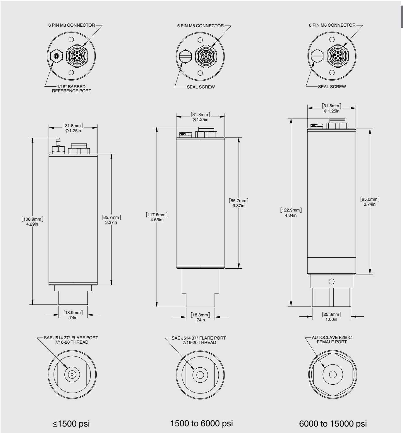
Figure 8.4 Technical Drawings
