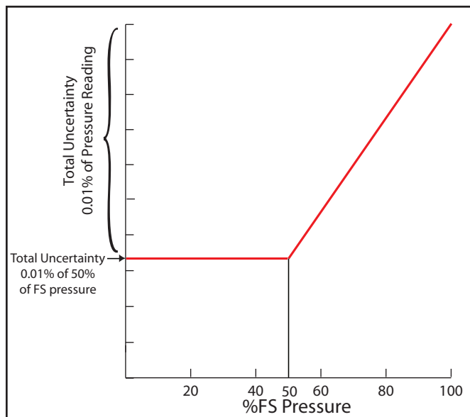
Figure 4.7.1a - IntelliScale IS-50
