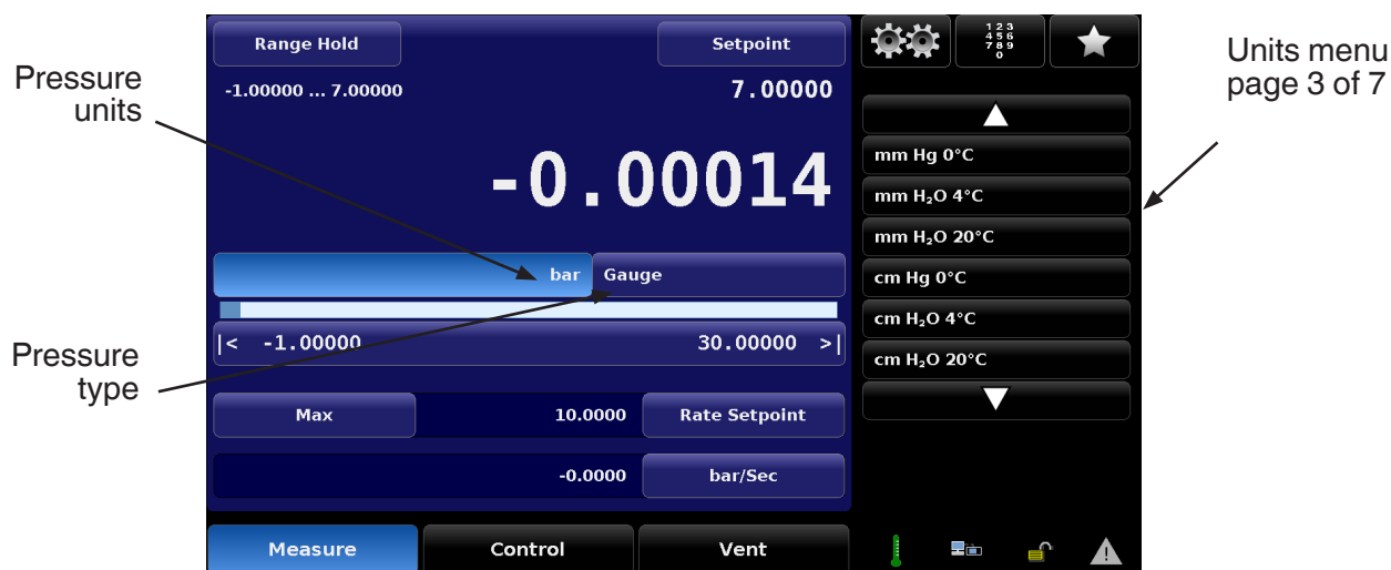
Figure 6.2.12 - Pressure Units
