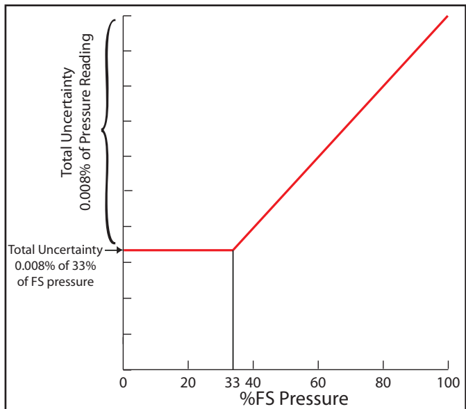
Figure 4.7.1b - IntelliScale IS-33
