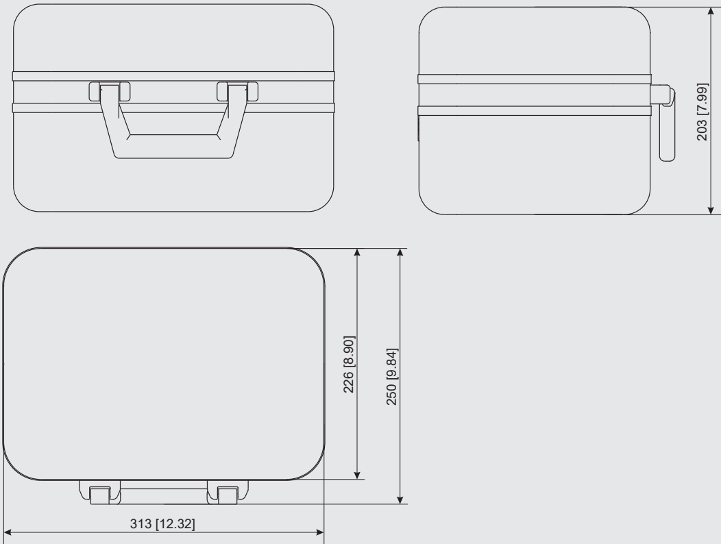
Case for model CPH8000-P1
