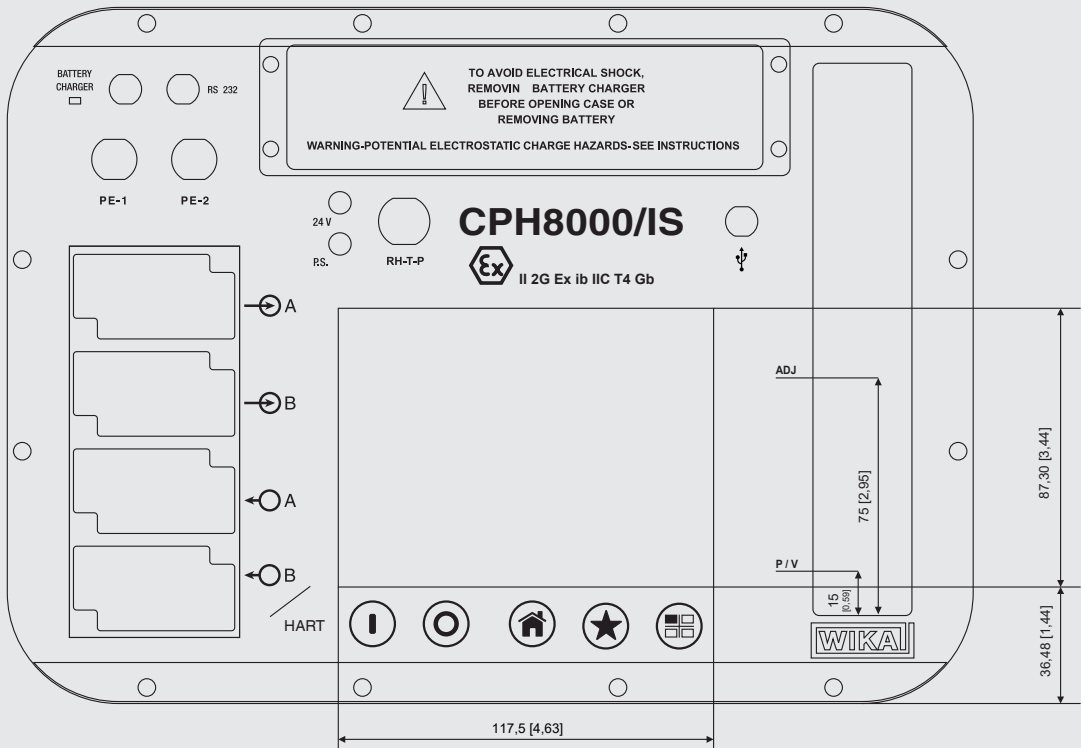
Front panel of model CPH8000-P1
