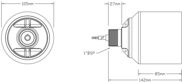
dB25 Transducer Drawing
