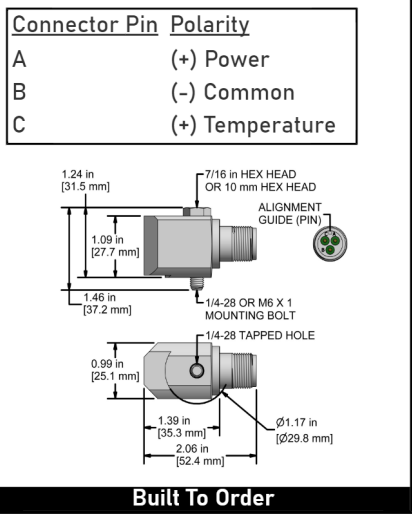
TC224-1A 3 Pin Connector
