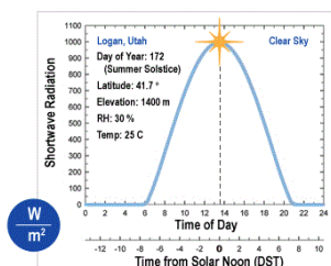
MODEL FOR PYRANOMETER
