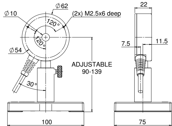
RM9-PD Sensor
