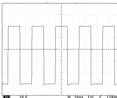
50% Duty Cycle, 50KHz, 50V, 10A, 5 Ohm Load
