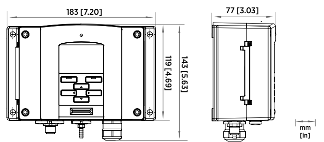
PTB330 dimensions
