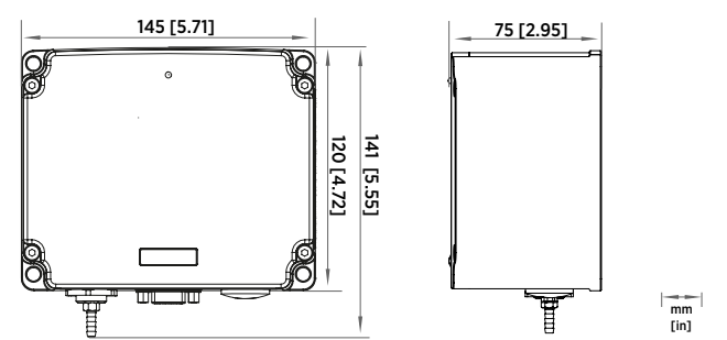
PTB330AWS dimensions
