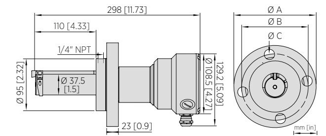
Dimensions PR53GP 2" flange
