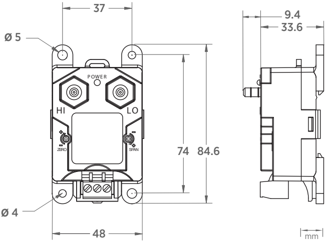
PDT101 dimensions
