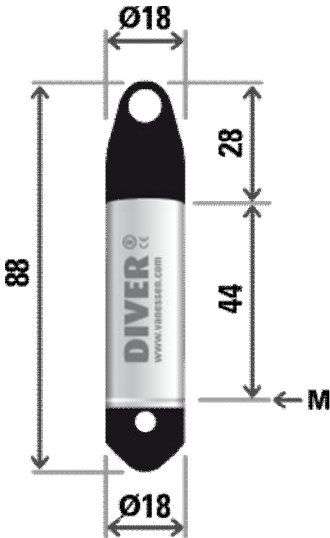
M = membrane Dimensions in mm
