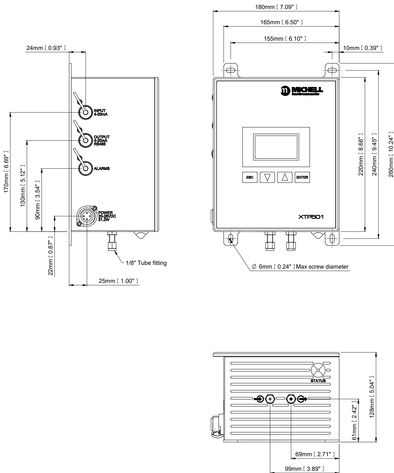
Figure 33 501 Dimensional Drawings – GP1
