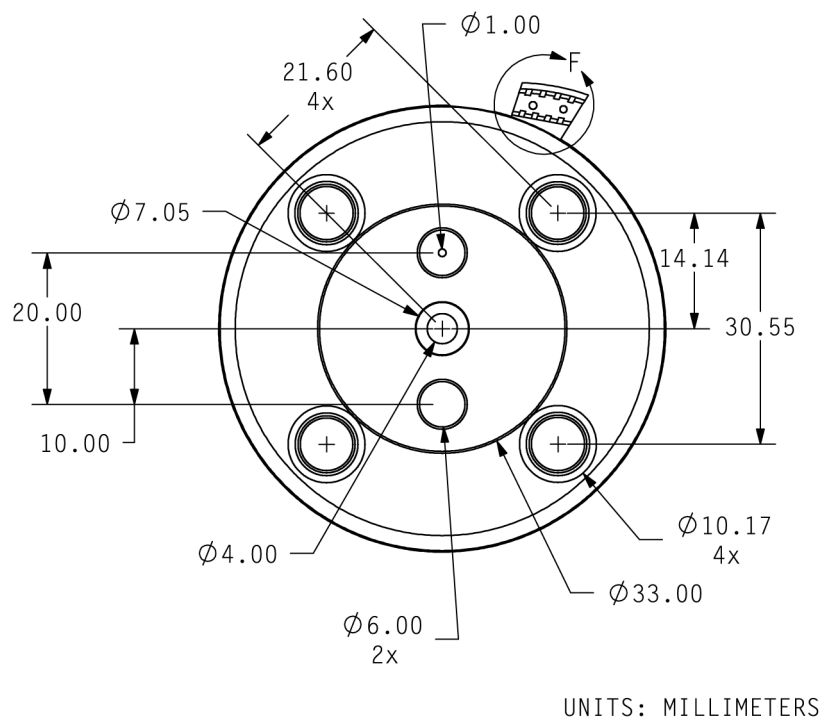
Figure 4a. GPS 18x Bottom Case Dimensions, Under Mold
