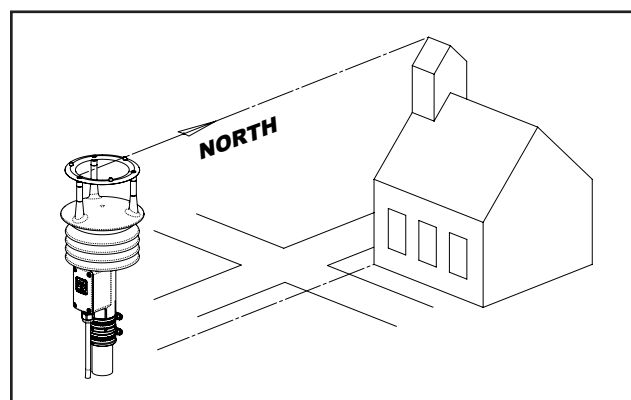
Fig 4.2.1 Sighting of Wind Sensor using Geographic Feature
