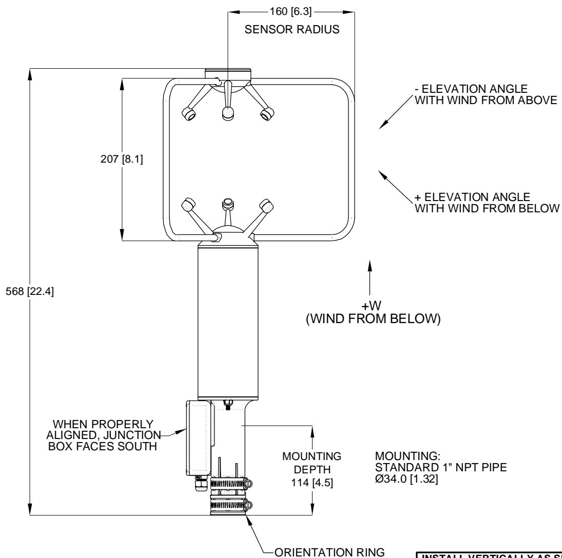
SIDE VIEW
